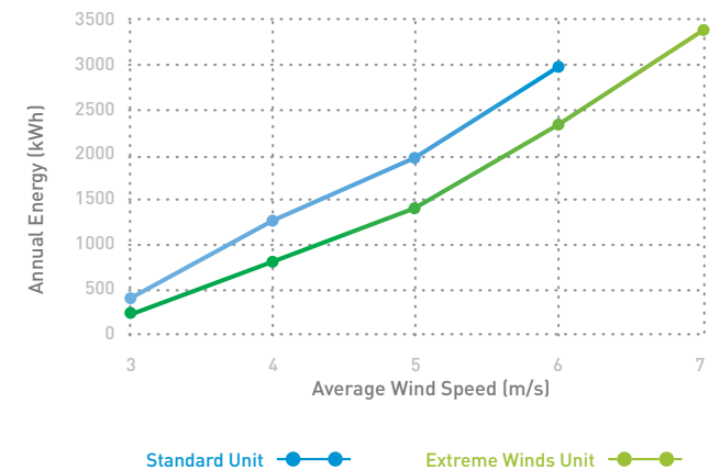
Windspire Annual Energy Production
